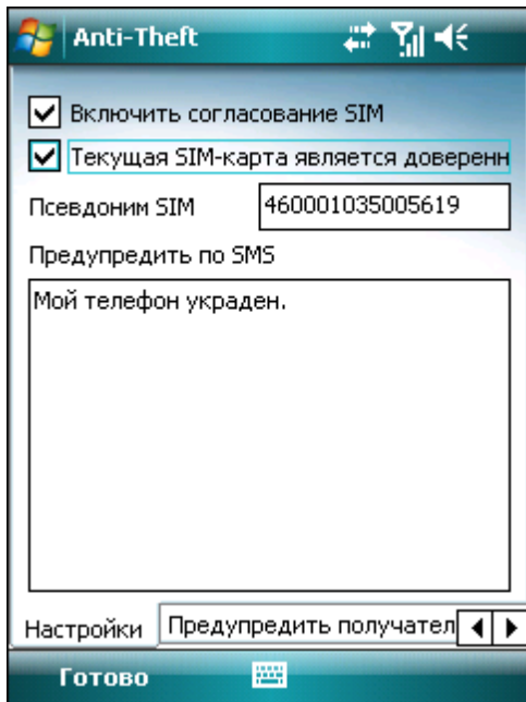
Anti-Theft настройки
